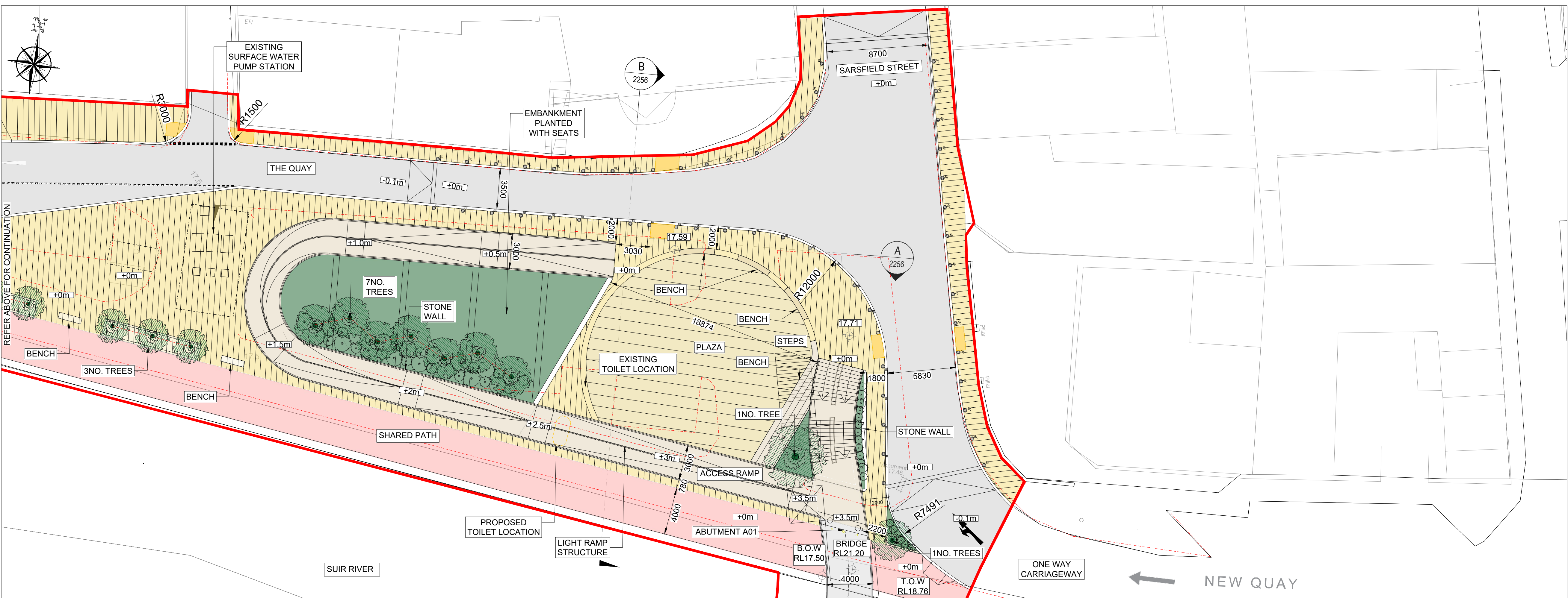
PLAN 2 SCALE 1:200
